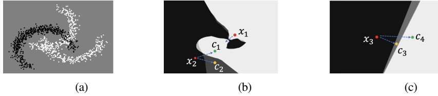
Figure 1: Illustration of the boundary change in a deep model (b) and a linear model (c) for a 2D dataset (a) when changing the seed for random initialization during the training. Shaded regions correspond to the area when two deep models in (b) (or two linear models in (c)) make different predictions.
