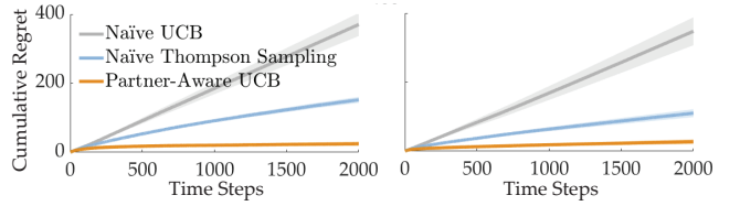
Figure 3: Cumulative regrets over 100 runs for different algorithms with (left) fixed and (right) random reward means.
