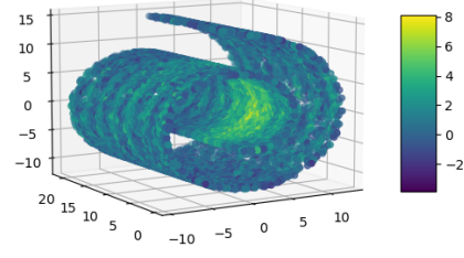
(b) Noisy observation
