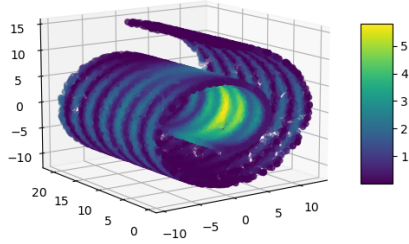
(a) Original function
