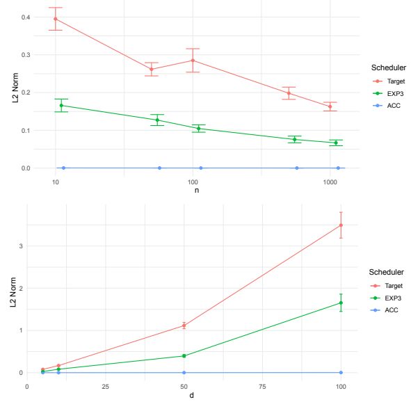
Figure 2. L_2 distance between the final estimate \theta_i and \theta_{t^*}^* under different total numbers of observations n and different numbers of dimensions d . The confidence intervals are the standard deviation of 1000 independent runs.
