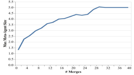
Figure 1: Average size of the largest meta-agent at the end of the search as a function of the number of merge operations that were performed by baseline ID+EPEA*
