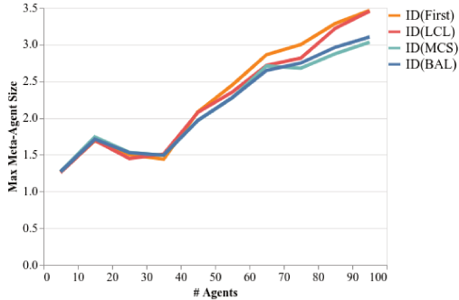
Figure 4: Average size of the largest meta-agent at the end of the search as a function of the number of agents in room maps from the MAPF benchmark
