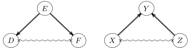
Figure 3: A priority graph for a PBS node with two meta-agents, each containing three agents and an internal conflict
