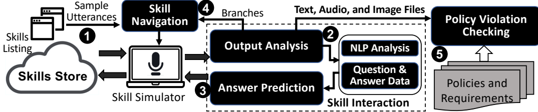
Figure 2: SKILLDETECTIVE overview.
