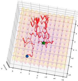
Figure 2. A typical BBI trajectory (starting from the circle) explores the rich landscape, stopping only at the global minimum (star).
