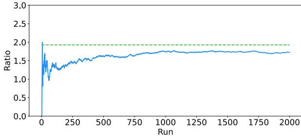
Figure 6. Partial ratios of convergence to the different basins on multiple runs (blue). All the runs start from the same initial point and are performed with N_b = 1 , \Delta t = 10^{-2} , T_1 = 750 , T_2 = 20 , \delta E = 0 , \Delta V = 10^{-3} . The asymptotic ratio is within 11% of the expected ratio for a mixing system (Eq. (18), green).
