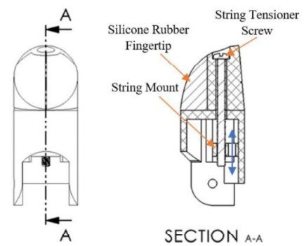
Figure 2. Cross-section of the distal and middle phalanx depicting the silicone rubber tip and the tendon tension mechanism. The string tensioner screw allows for the string mount to move up and down (motion given by the blue arrows) so that the string to be easily tensioned.
