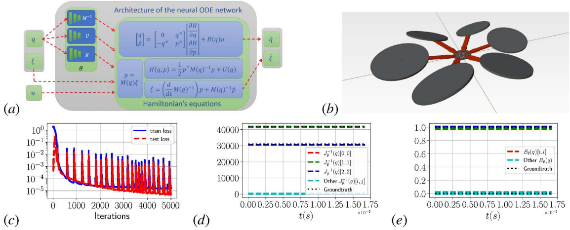
Figure 1: SE(3) Hamiltonian neural ODE network: (a) network architecture, (b) simulated hexarotor for evaluation, (c) training loss, (d) learned inverse inertia \mathbf{J}_\theta(q)^{-1} , and (e) learned input matrix \mathbf{B}_\theta(q) along a test trajectory, evaluated on the simulated hexarotor.
