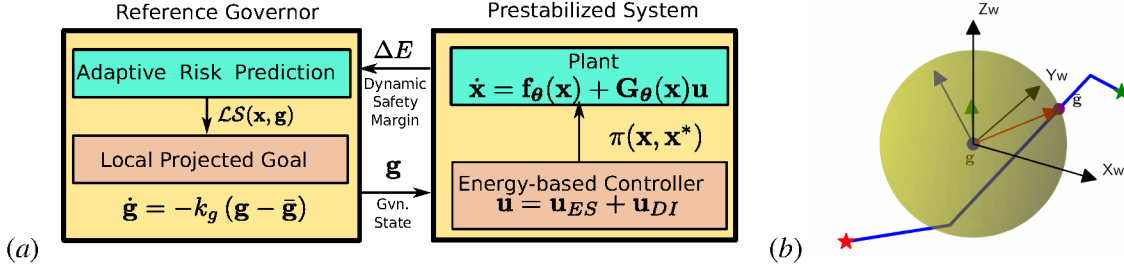
Figure 2: (a) Structure of the reference-governor tracking controller: a reference governor with state \mathbf{g} adaptively tracks a point \bar{\mathbf{g}} along the desired path \mathbf{r} and generates a time-varying equilibrium \mathbf{x}^* = \ell(\mathbf{g}, \bar{\mathbf{g}}) for the closed-loop Hamiltonian system; (b) A local projected goal \bar{\mathbf{g}} (purple dot) is generated as the furthest intersection between the local safe set \mathcal{LS}(\mathbf{x}, \mathbf{g}) (yellow sphere) and the path \mathbf{r} (blue curve). Given \mathbf{g} and \bar{\mathbf{g}} , a desired equilibrium \mathbf{x}^* = \ell(\mathbf{g}, \bar{\mathbf{g}}) is generated for the Hamiltonian system with orientation indicated by the red, green, and blue arrows, respectively.
