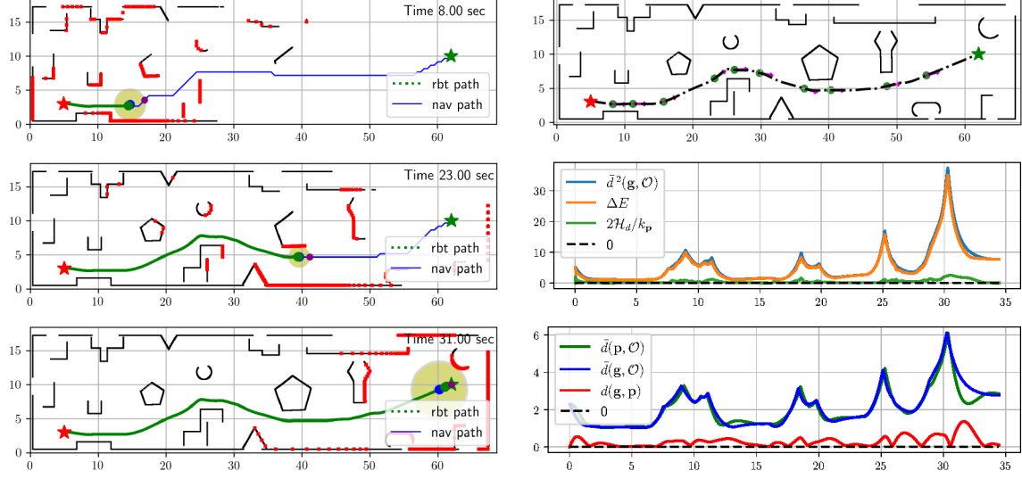
Figure 3: Safe tracking control for a hexarotor aerial robot in an unknown cluttered environment. The hexarotor (green dot) navigates from a start location (red star) to a goal location (green star) while avoiding obstacles. The obstacles are sensed by a simulated LiDAR sensor (red points). On the left are snapshots of the environment showing the robot (green dot), lidar scans (red dots), and the unsafe set \mathcal{O} (black surfaces) at different times. The reference path (blue curve) is re-planned online from the governor position (blue dot) to the goal (green star) using an A^* algorithm. The local projected goal \bar{\mathbf{g}} (purple dot) is computed based on the obstacle distance (gray ball) and the local safe set (yellow ball). On the upper right, the robot's heading (purple arrow) are plotted along the path. The middle right figure shows the dynamic safety margin \Delta E in (12) and the scaled desired Hamiltonian 2\mathcal{H}_d(\mathbf{x}, \mathbf{x}^*)/k_p while the lower right figure plots the distance to the obstacles d(\mathbf{p}(t), \mathcal{O}) (green curve), showing that the safety constraints are never violated.
