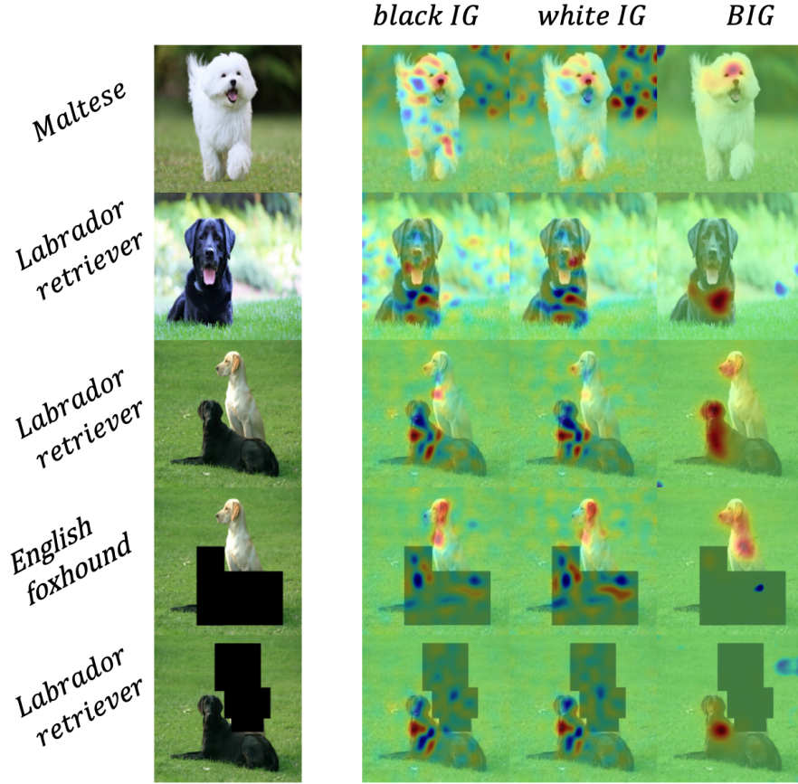
Figure 12: Full results of Fig. 7 in Sec. 6. For the third, fourth and fifth example, we compute the attribution scores towards the prediction of the third example, Labrador retriever . IG with black or white attributions show that masked area contribute a lot to the prediction while BIG “accurately” locate the relevant features in the image with the network’s prediction.
