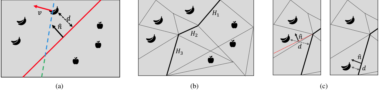
Figure 2: Different classifiers that partition the space into regions associated with apple or banana . (a) A linear classifier where \hat{n} is the only faithful explanations and v is not. (b) A deep network with ReLU activations. Solid lines correspond to decision boundaries while dashed lines correspond to facets of activation regions. (c) Saliency map of the target instance may be normal to the closest decision boundary (right) or normal to the prolongation of other local boundaries (left).
