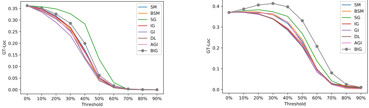
Figure 13: GT-Loc scores for different attributions. GT-Loc measures the portion of instances where the IoUs of between the groundtruth bounding box and the bounding box generated by thresholded the attributions are greater than 0.5. The x-axis is the percentile used to threshold an attribution map to determine the highlighted area and y-axis is the GT-Loc score aggregated over all the instances. Left: Standard ResNet50. Right: Robust ResNet50( \ell_2|0.3 ). Note that Fig. 13 is a collection of Fig. 5 and 6 from Sec. 5.
