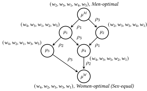
Figure 1: The stable lattice for the profile described in Example 1.1 with six stable solutions. Matchings are denoted as lists of women matched to men according to their indices, rotations are indicated by \rho_x on arcs.
