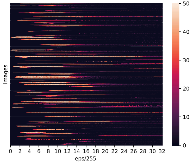
Figure 7: The maximum number of times that the prediction was changed to a class, throughout the process of perturbing each of the 512 image before success using Auto-PGD with CW loss against DSL+20.
