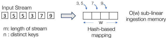
Figure 5: Hashing enables sub-linear memory complexity
