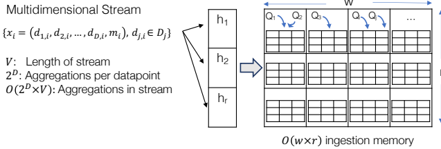
Figure 8: Redundant sketch vectors and pairwise-independent hashes for tighter error bounds.
