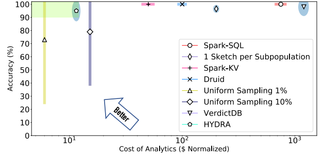
Figure 1: End-to-end cost of analytics. The green-shaded region indicates the ideal operating regime for HYDRA.
