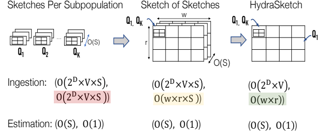
Figure 3: Comparison of Ingestion and Estimation (CPU time, space complexity) for different sketch-based designs. We highlight the theoretical improvements in space complexity from HYDRA’s design ideas.
