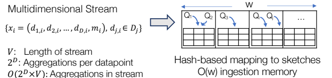
Figure 7: Hash-based mapping of subpopulations to a sketch vector.
