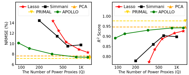
Figure 12: Per-cycle power accuracy vs number of proxies for per-cycle power prediction (Cortex-A77).
