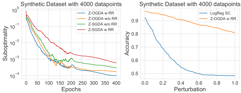
Figure 2: Experimental results for a synthetic dataset with n = 4000 . (Left pane)) Suboptimality iterates generated by the four algorithms (A-I), (A-II), (A-III), (A-IV), respectively denoted as Z-OGDA w RR, Z-OGDA w/o RR, Z-SGDA w RR, Z-SGDA w/o RR. (Right pane) Comparison between decay in accuracy of strategic classification with logistic regression (trained with \zeta = 0.05 ) and Alg. (A-I) with changes in perturbation.
