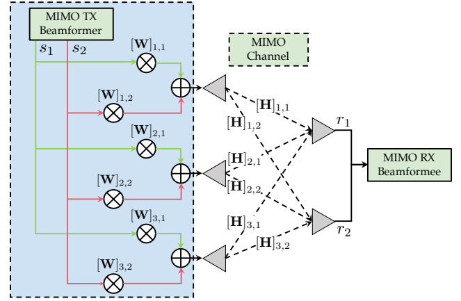
Fig. 2: 3 \times 2 MIMO system. The grey triangles represent the antennas. s_1, s_2 and r_1, r_2 stand for the transmitted and received signals respectively. \mathbf{W} is the steering matrix containing the weights to shape the beams. \mathbf{H} is the CFR.
