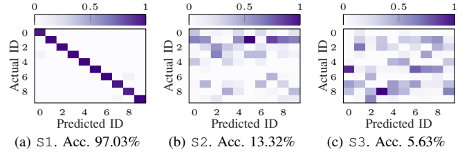
Fig. 15: Confusion matrices, beamformee 1, 3 TX antennas, spatial stream 1.
