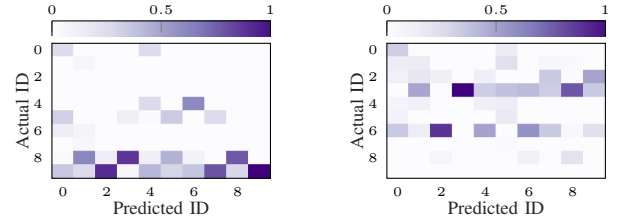
(a) Train on beamformer 1 and testing on beamformer 2. Acc. 25.86% (b) Train on beamformer 2 and testing on beamformer 1. Acc. 25.02%
