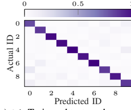
(a) S4. Train and test on the complete AP mobility path. Acc. 82.56%
