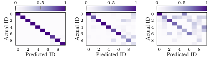
(a) S1. Acc. 98.02% (b) S2. Acc. 75.41% (c) S3. Acc. 42.97%
