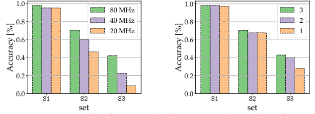
(a) Accuracy by varying the channel bandwidth, i.e., selecting respectively N_{\text{col}} = 234, 110, 54 , out of the K = 234 OFDM sub-channels. (b) Accuracy by varying the no. of transmitter antennas, i.e., selecting respectively N_{\text{ch}} = 3, 2, 1 rows of the beamforming feedback matrix \hat{\mathbf{V}} .
