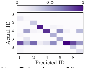
(b) S4. Train and test on different AP mobility sub-paths. Acc. 41.15%
