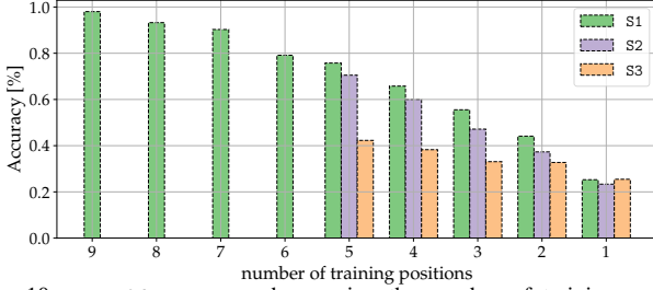
Fig. 10: DeepCSI accuracy by varying the number of training positions from the considered set (see Table I). Set S1 is trained on a maximum of 9 beamformer positions while S2 and S3 on 5.
