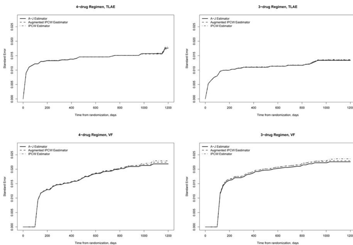
Figure 2. Standard Errors of \hat{F}_j(t) , by Regimen and Type of Failure, using Bootstrap Variance Estimation.
