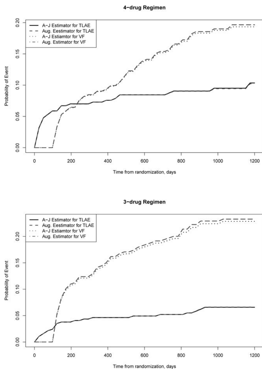
Figure 1. Cumulative Incidence Curves, by Regimen.
