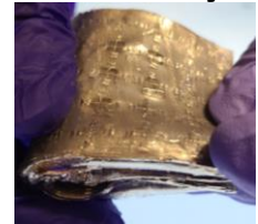
Figure 5. Physical flexibility demonstration of the fabricated metasurface.
