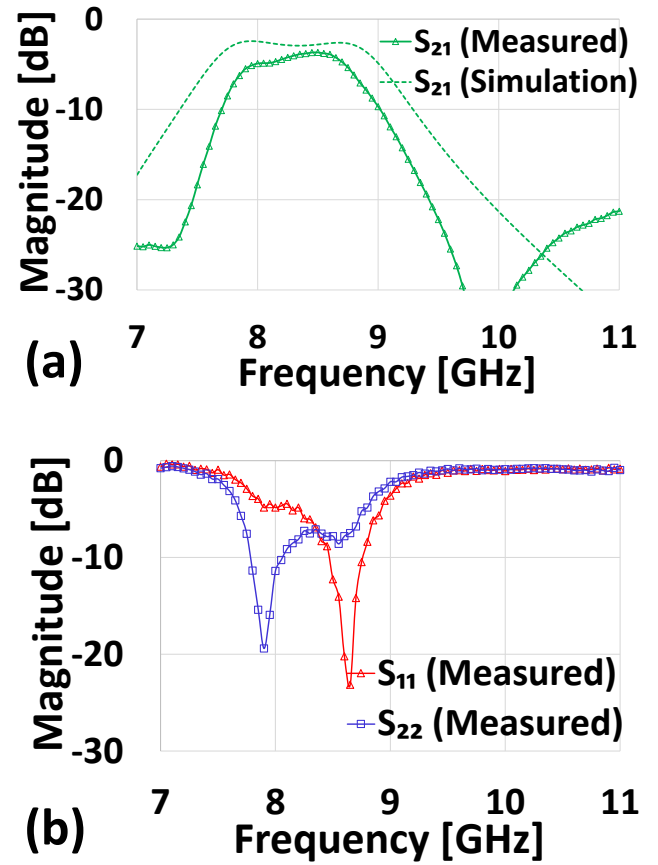
Figure 7. WR-90 waveguide results for band-pass metasurface. (a) Simulated and measured transmission coefficient. (b) Measured reflection coefficients.
