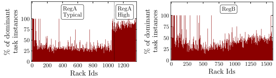
Figure 11: Dominant task density across racks.
