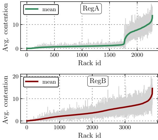
Figure 12: The variation of average contention across racks for different regions.
