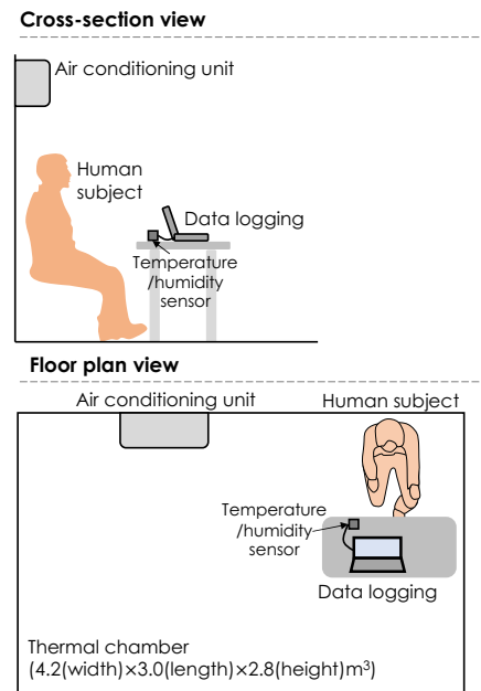
Figure 3. Cross-section and floor-plan views of the experimental testbed.
