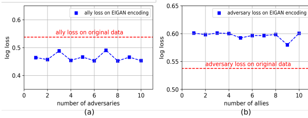
Figure 6: EIGAN’s effect of the number of (a) adversaries, and (b) allies on the testing loss for MIMIC-III. The ally/adversary objectives are chosen as different attributes from the source. The achievable loss is reasonably constant and is not affected by addition of more allies/adversaries.
