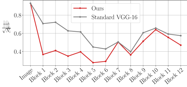
Figure 2: HaH blocks yield sparser activations than baseline. The measure of sparsity is the Hoyer ratio (Hoyer, 2004) of \ell_1 norm to \ell_2 norm of activations across channels, averaged across spatial locations, and then normalized to lie in [0,1] (lower values correspond to more sparsity).
