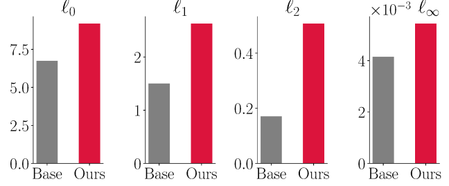
Figure 5: The average norm of minimum-norm adversarial attacks is higher for our model for all \ell_p norms considered.
