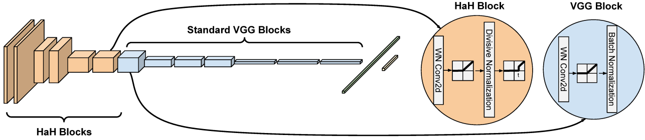
Figure 1: Our model consists of two different types of blocks: first 6 blocks are Hebbian-anti-Hebbian (HaH) while the rest are regular VGG blocks. HaH blocks use a weight normalized convolutional layer, followed by ReLU, divisive normalization and thresholding. Regular VGG blocks use a weight normalized convolutional layer followed by ReLU and batch norm.
