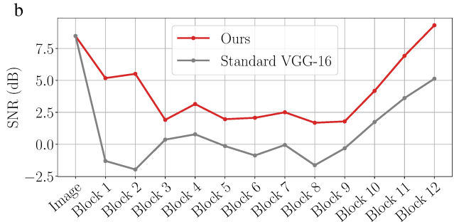
Figure 3: a: To compute the SNR at the n^{\text{th}} block inputs, we divide the \ell_2 norm of the block input corresponding to clean image by the \ell_2 norm of the difference of block corresponding to clean and noisy images. b: Comparison of SNR values of the block inputs for the standard base model (gray) and ours (red).
