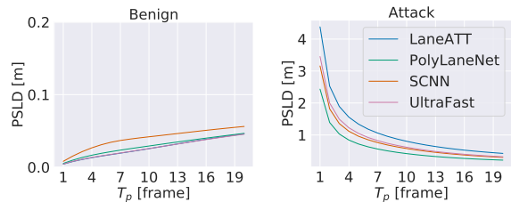
Figure 5. PSLD for the 4 major lane detection models when T_p is varied from 1 to 20 frames in the benign and attack scenarios.
