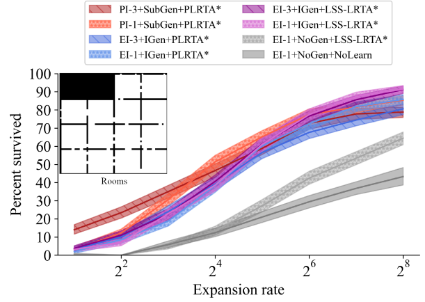
Figure 1: Experimental results, the solid lines are measured success rate with the area between the 5th and 95th percentile shaded, determined by bootstrapping with n = 1024 .
