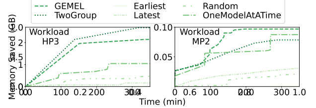
Figure 16: Comparing variants of Gemel’s merging heuristic on two representative workloads.
