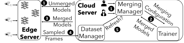
Figure 9: Gemel architecture.
