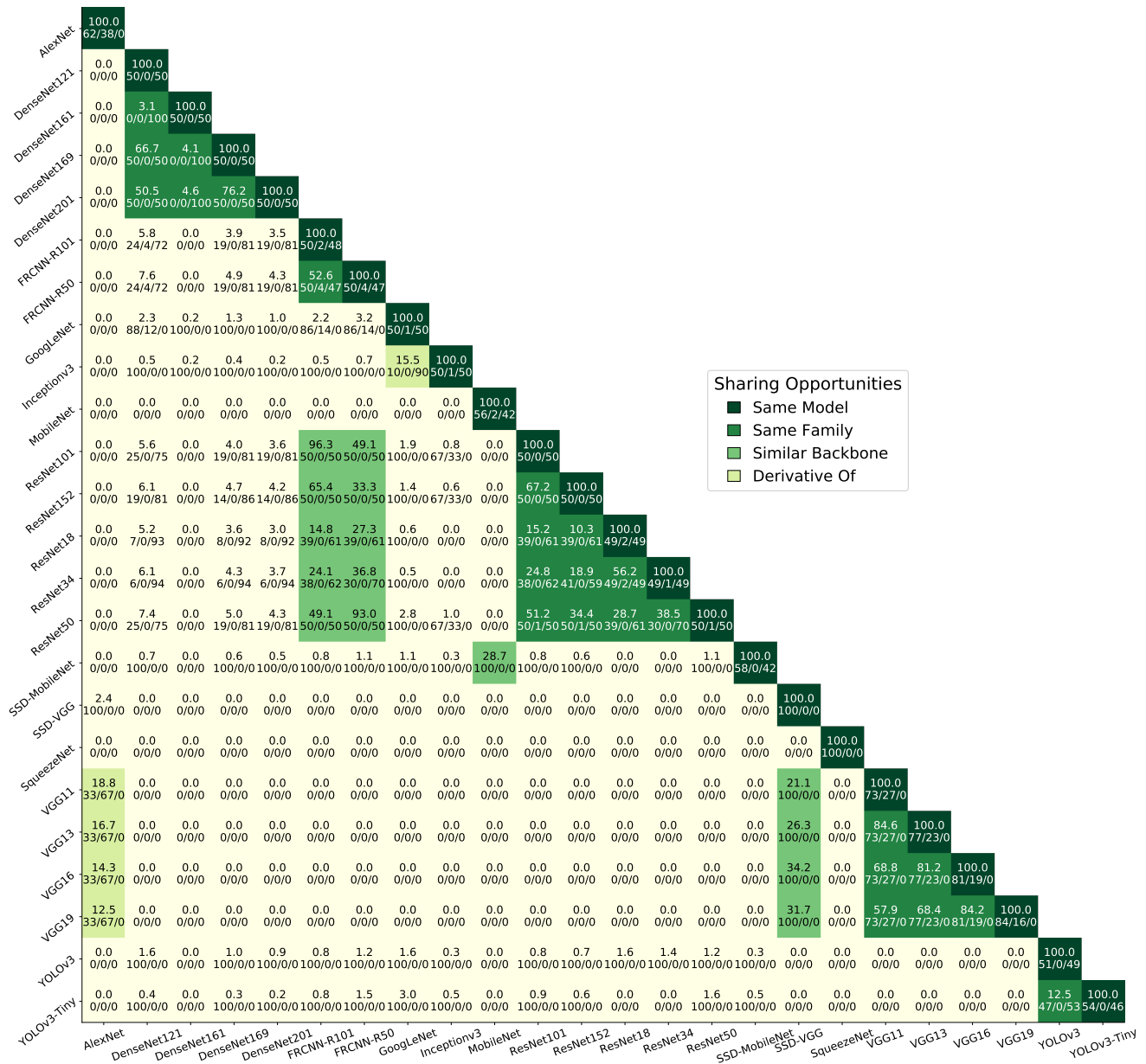
Figure 20: Extended version of Figure 4. For each unique pair of models, we show the percentage of architecturally identical layers and of those layers, the percent breakdown across layer types (% Convolutional / % Linear / % BatchNorm).
