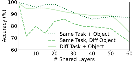
Figure 8: Accuracy after 5 hours of retraining when sharing additional architecturally-identical layers for different model pairs (starting from their origins). Tasks cover detection (Faster RCNN) and classification (ResNet50), and two objects: people, vehicles. Results list the lower per-model accuracies per pair.
