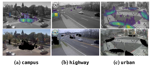
Figure 3: (Top) Heatmap measuring the maximum time any object spent in each pixel, normalized to the max (yellow) per video. (Bottom) The resulting masks used for our evaluation, chosen from the list of masks automatically generated using the algorithm in §I of [33].
