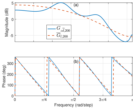
Fig. 4. Comparison of the frequency response of G_{zd,200} with that of \bar{G}_{f,200} . The magnitude plots and the phase plots match approximately.
