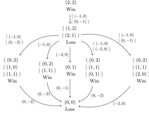
■ Figure 1 Winning strategy for current player in QUANTUM NIM (2, 2) , showing that quantum moves impact the game’s outcome. (There are four additional move options from \langle (1, 2) | (2, 1) \rangle that are not shown because they are symmetric to moves given.)
