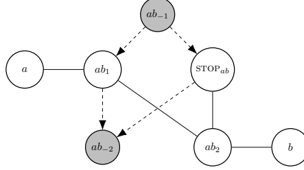
■ Figure 3 Gadget for a GEOGRAPHY edge (a, b) in UNDIRECTED GEOGRAPHY. Prior to the current position, the quantum moves ab_{-1} \rightarrow \langle ab_1 \mid \text{STOP}_{ab} \rangle \rightarrow ab_{-2} were made.
