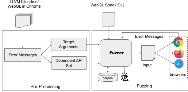
Figure 2: GLeeFuzz design. In the pre-processing stage, GLeeFuzz identifies error messages, and computes their target arguments and the dependent API set, which the fuzzer uses for error message guided input mutations.
