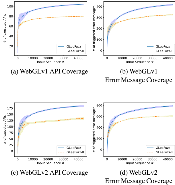
Figure 3: Coverage comparison between GLeeFuzz and GLeeFuzz-R in metrics of the number of executed APIs and the number of triggered error messages.
