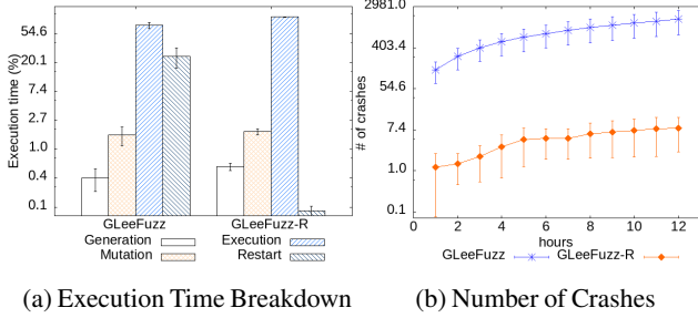
Figure 4: Execution time and crash comparison between GLeeFuzz and GLeeFuzz-R. The y-axes show log scale.
