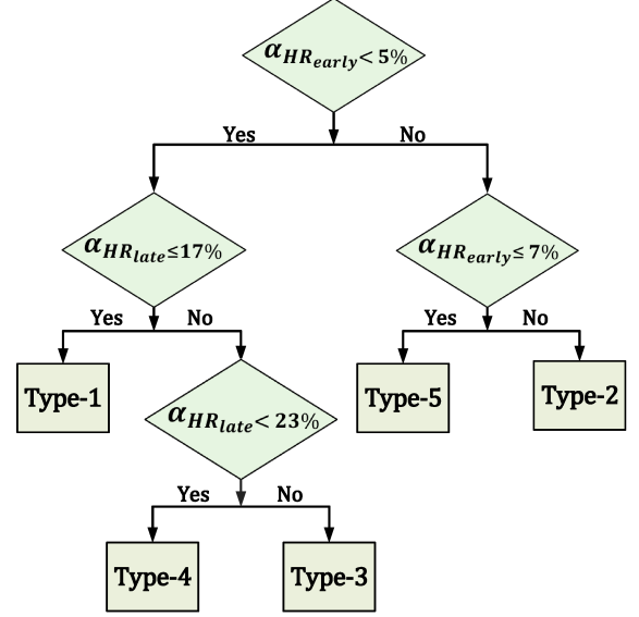
Fig. 4. Flowchart of classification algorithm for HR shapes
