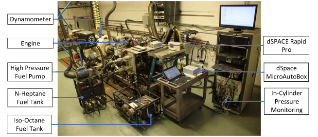
Fig. 2. RCCI engine setup
