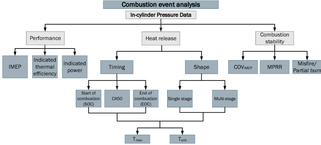
Fig. 1. Combustion metrics
