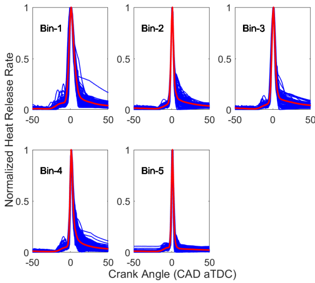
Fig. 6. K-means classification of heat release rate traces
