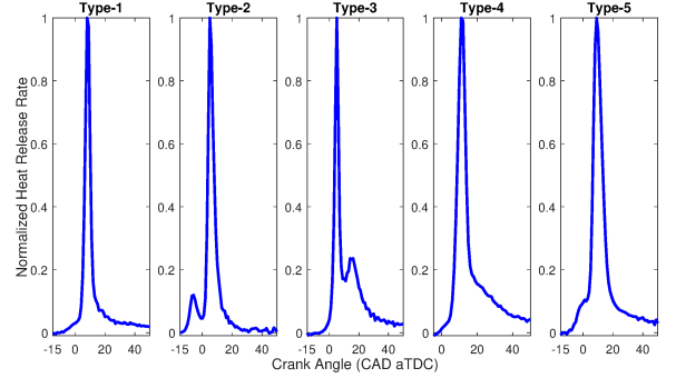
Fig. 5. Identified shapes of heat release rate traces
