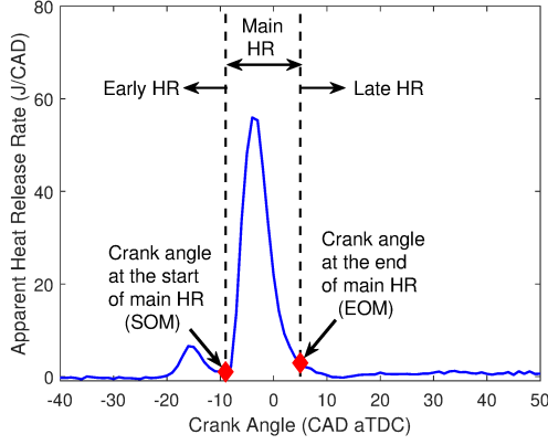
Fig. 3. Crank angles showing early, main and late heat release (HR)
