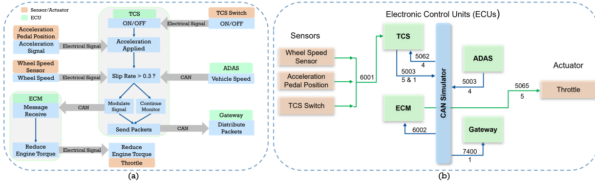
Figure 1. Traction Control system (a) platform's functionality flow diagram and (b) platform's primary system design
