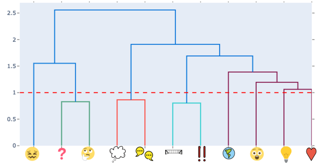
Figure 3: Hierarchical clustering of the emoji based on the model's prediction. The dashed red line represents the confidence threshold.
