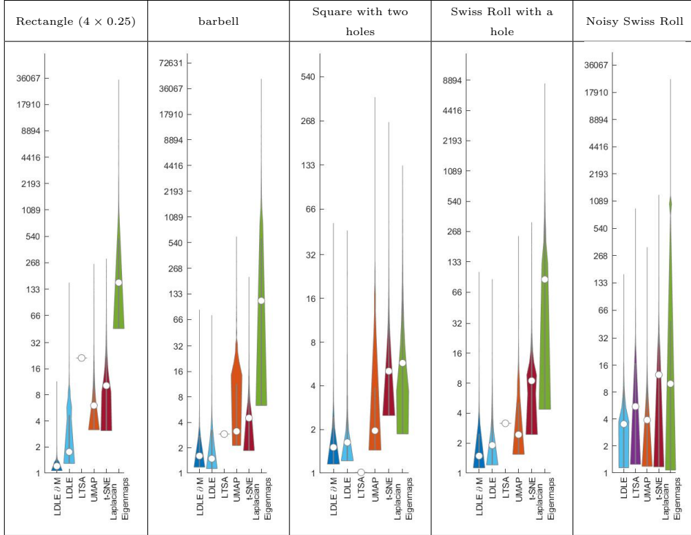
Figure 16: Violin plots (Hintze and Nelson, 1998; Bechtold et al., 2021) for the distribution of \mathcal{D}_k (See Eq. (64)). LDLE \partial\mathcal{M} means LDLE with boundary known apriori. The white point inside the violin represents the median. The straight line above the end of the violin represents the outliers.
