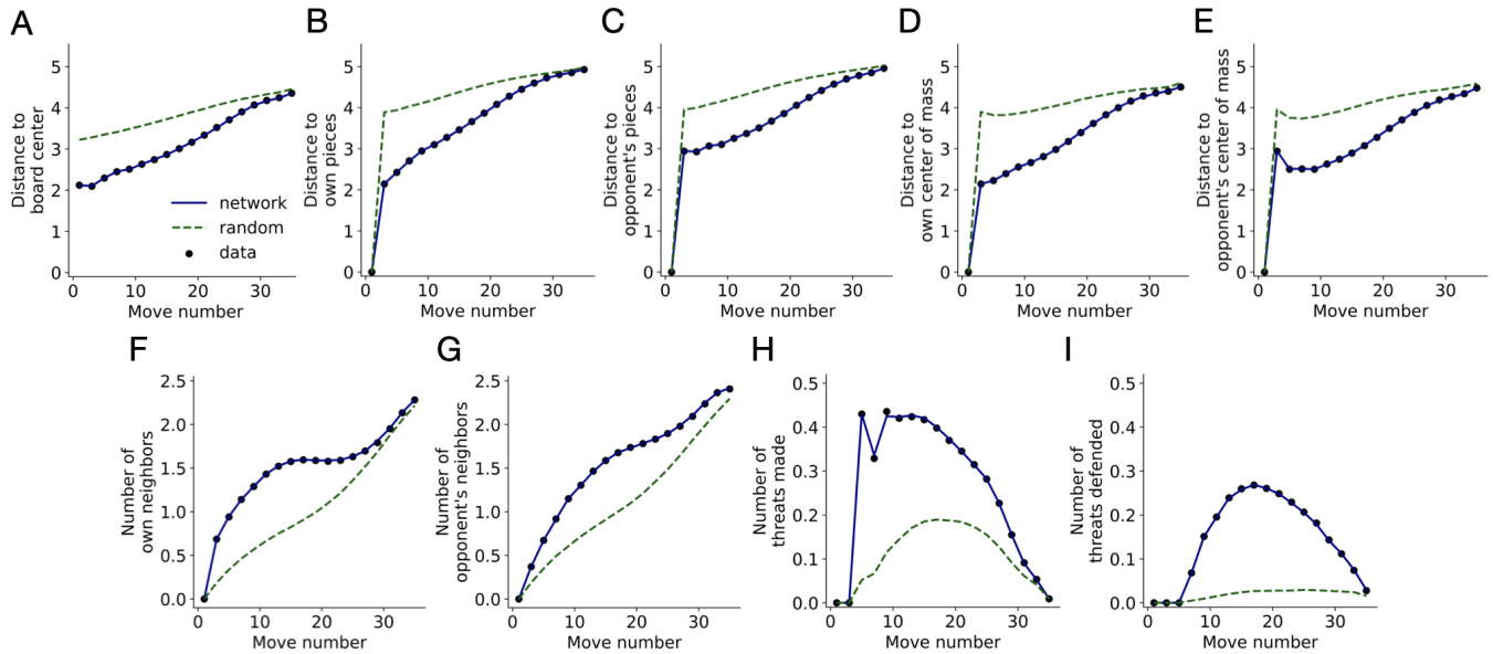
Figure 5: Summary statistics as validation of the neural network's performance. Each statistic is averaged by move number for moves made by users (black circles), the neural network (blue lines), or random moves (green dashed lines).
