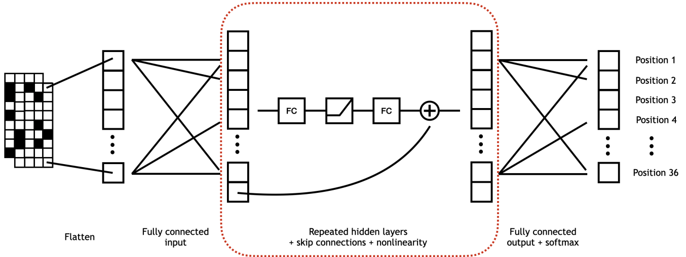
Figure 2: Neural network architecture. The board is represented as a 2 \times 4 \times 9 tensor filled with zeros where there are no pieces and ones where there are pieces. One matrix encodes the user’s pieces, and the second encodes the AI agent’s pieces. The board representation is flattened to a 72 dimensional vector, and then passed into a series of hidden layers. Each hidden layer contains a fully connected layer, a nonlinearity, another fully connected layer, and then adds the input from the skip connections. Finally, the fully connected output layer has 36 units and is passed through a softmax function, which gives the probability that the model assigns to the human player selecting each position of the board. In addition to varying the number of hidden layers in the network, the number of units per fully connected layer is also varied when testing different networks.
