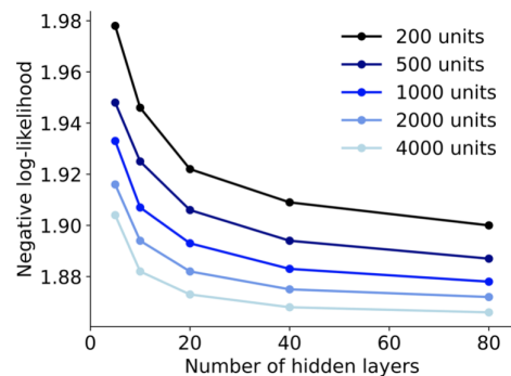
Figure 4: Scaling up the neural network achieves an upper bound on goodness of fit. Log-likelihood on the test data set as a function of the number of hidden layers and number of units per hidden layer in each network.
