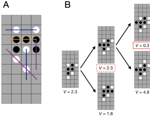
Figure 3: Planning model specification. (A) Features used in the heuristic function. Features with identical colors are constrained to the same weights. (B) Illustration of the best-first search algorithm. In the root position, black is to move. After expanding the root node with two candidate moves for black and evaluating the resulting positions using the heuristic function, the algorithm selects the highest value node ( V = 2.3 ) on the second iteration and expands it with two candidate moves for white. The algorithm evaluates the resulting positions, and backpropagates the lowest value ( V = 0.3 ), since white is the opponent. This will be compared against alternatives in each intermediate node of the tree to decide in which direction to expand the tree on the next iteration.
