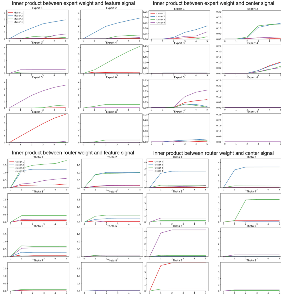
Figure 4: Mixture of nonlinear experts. Growth of inner product between expert/router weight and center/feature vector.
