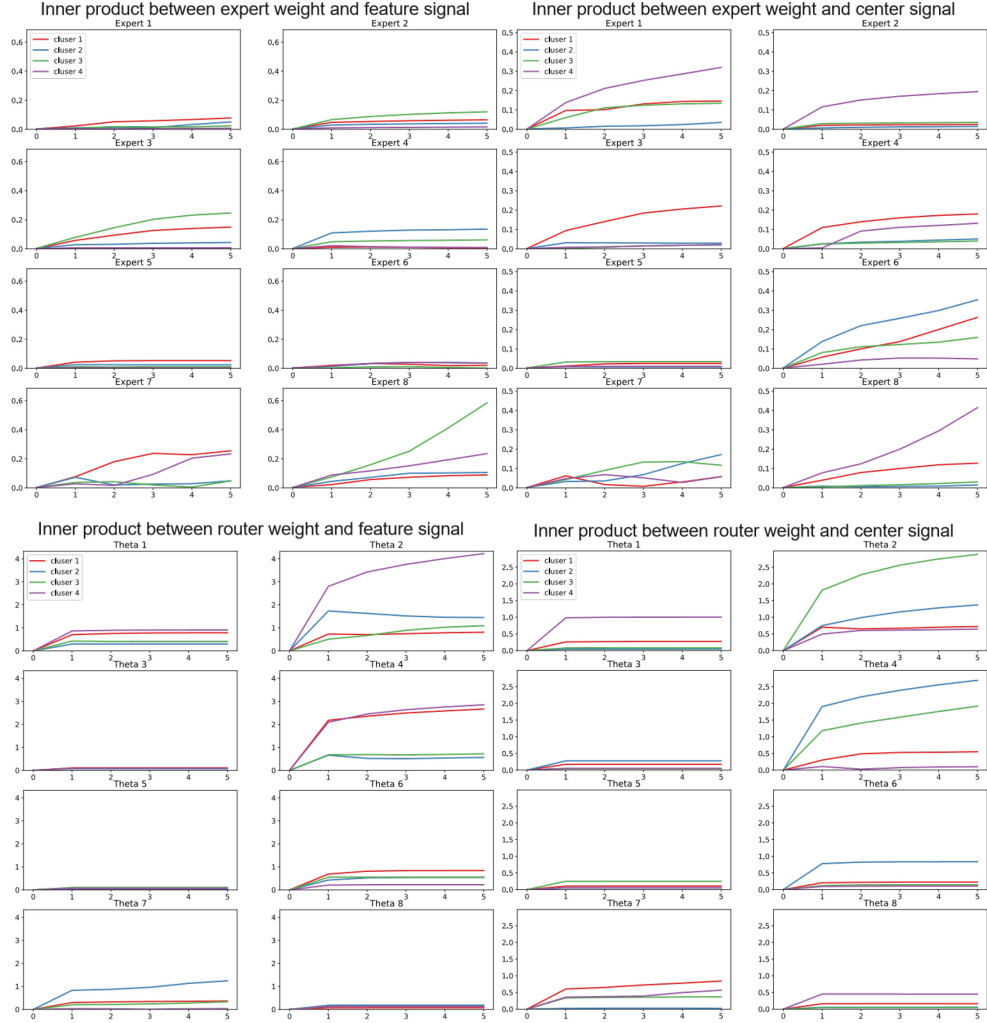
Figure 5: Mixture of linear experts. Growth of inner product between expert/router weight and center/feature vector.
