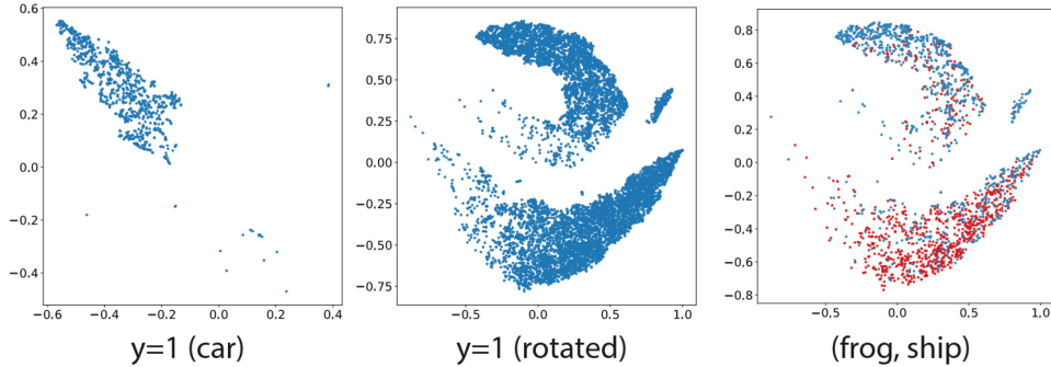
Figure 7: Visualization of the latent embedding on CIFAR-10 and CIFAR-10-Rotate with fixed label y . The left figure denotes the visualization of CIFAR-10 when label y is fixed to be 1 (car). The central figure represents the visualization of CIFAR-10-Rotate when label y is fixed to be 1 (rotated). On the right figure, red denotes that the data is from the ship class, and blue denotes that the data is from the frog class.
