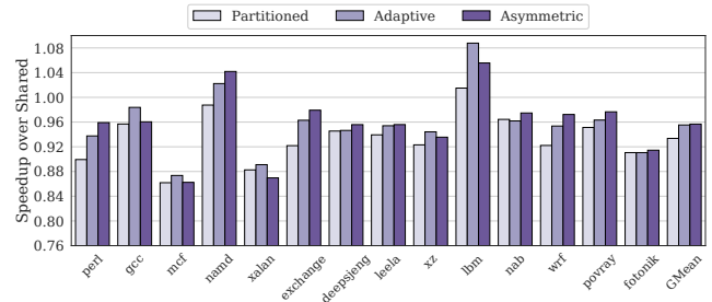
Figure 10: Partitioning Schemes for Fetch Bandwidth.
