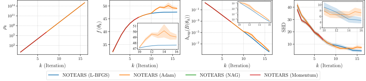
(a) NOTEARS.
