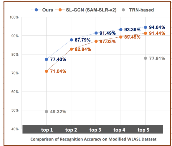
Figure 8: Comparison of recognition accuracy of our GCN-based method with another GCN-based method and with a CNN-based method.
