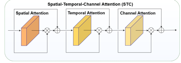
Figure 5: The STC Attention mechanism. The 3 sub-modules are arranged in the order: Spatial before Temporal before Channel attention. The generated attention maps are multiplied with the original feature maps. The residual connection in each attention sub-module is added to stabilize the training.
