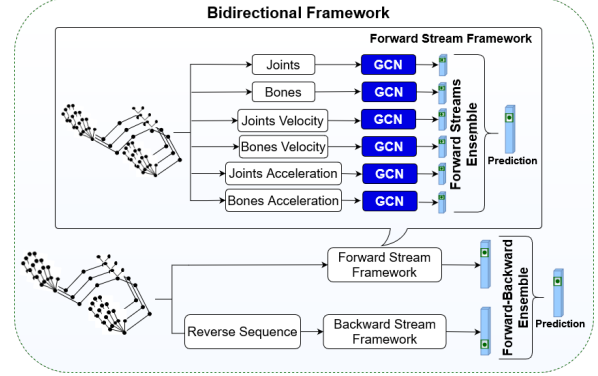
Figure 7: Illustration of our bidirectional framework.
