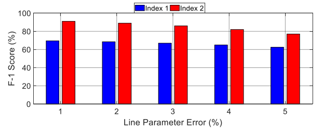
Figure 13: The performance of the MaDIoT 2.0 attacks versus the mean error in the New England power grid line parameters.
