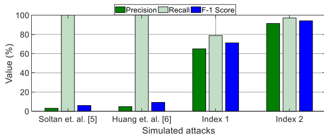
Figure 6: The performance of the proposed attack methods along with the approaches developed in the most recent works obtained from the New England power grid [5, 6].
