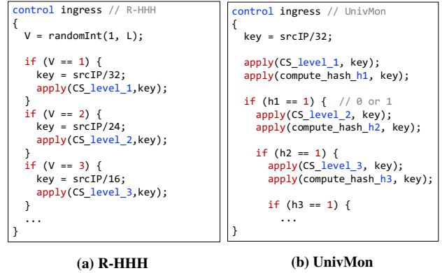
Figure 2: Simplified P4 code of existing multi-level sketches.
