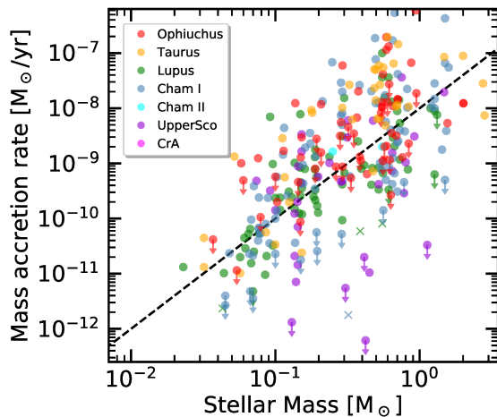
Fig. 4.— \dot{M}_{\text{acc}} vs M_{\star} for the targets for which both quantities are available in Table 1. The dashed line shows the \dot{M}_{\text{acc}} \propto M_{\star}^2 line, plotted to guide the eye, but it does not represent a fit to the data.
