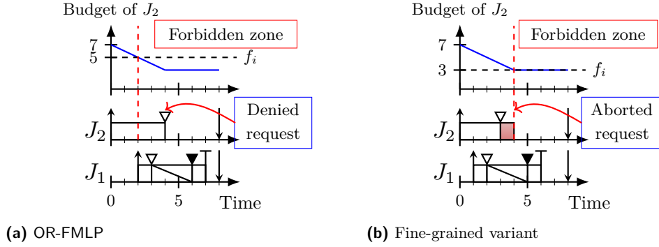
■ Figure 5 Illustration of FZs. Overheads/delays other than spinning are omitted to avoid clutter.
