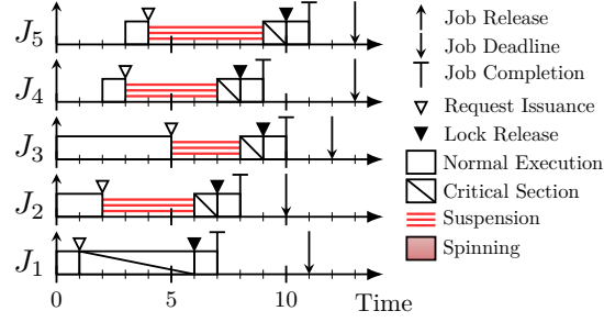
Figure 2 Jobs issuing requests to the global OMLP with m = 3 . (The notation in this figure is also used in subsequent figures.)
