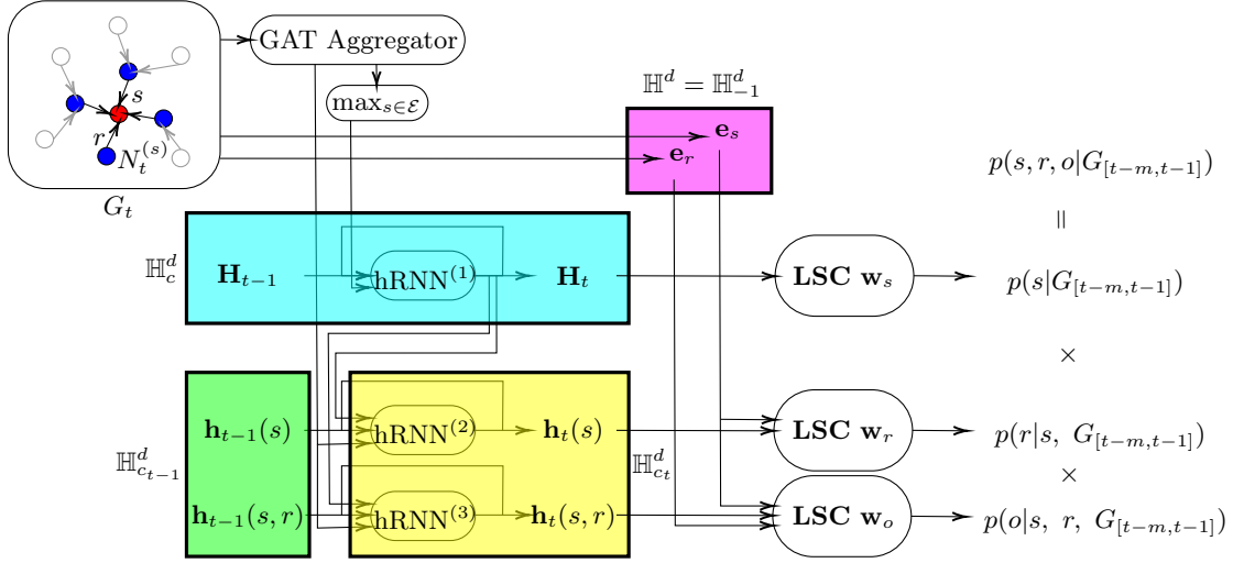
Figure 2: The overall architecture of HyperVC . Colored boxes are the hyperbolic spaces that contain the hyperbolic representations with designated curvatures. LSC \mathbf{w} refers to the linear softmax classifier parametrized by \mathbf{w} . Through the cyan box of the global representations, the green and yellow boxes of the local representations, and the pink box of time-consistent hyperbolic embeddings of entities and relations, we calculate the probability of triplet (s, r, o) at the timestamp t .
