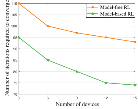
Fig. 3. Number of iterations required to converge vs. the number of devices.
