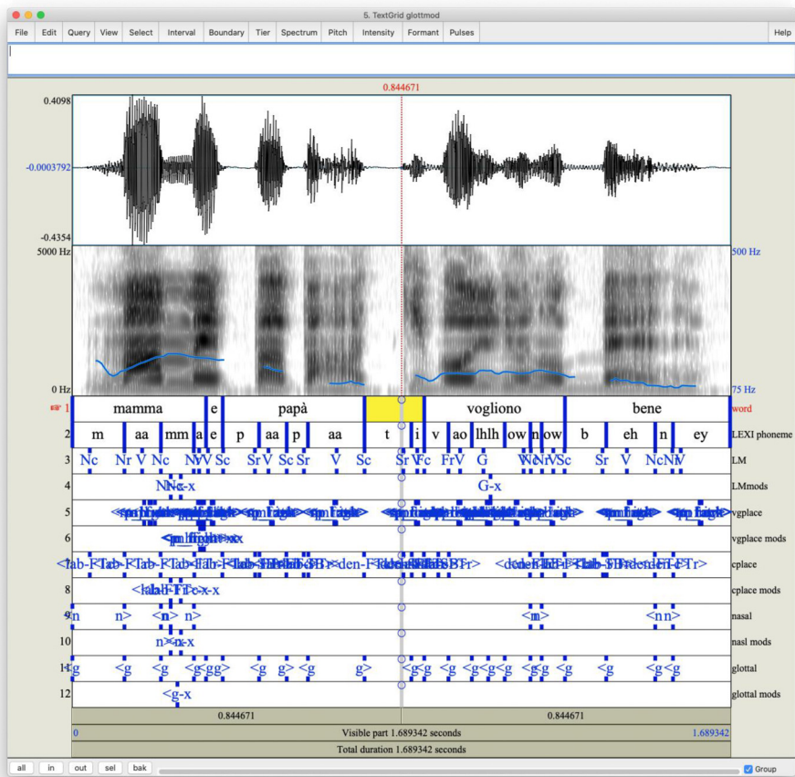
Fig. 2. Example of Praat output for sentence LDN_036_v1, including waveform and corresponding spectrogram computed from the .wav file and labeling information stored in the TextGrid file.
