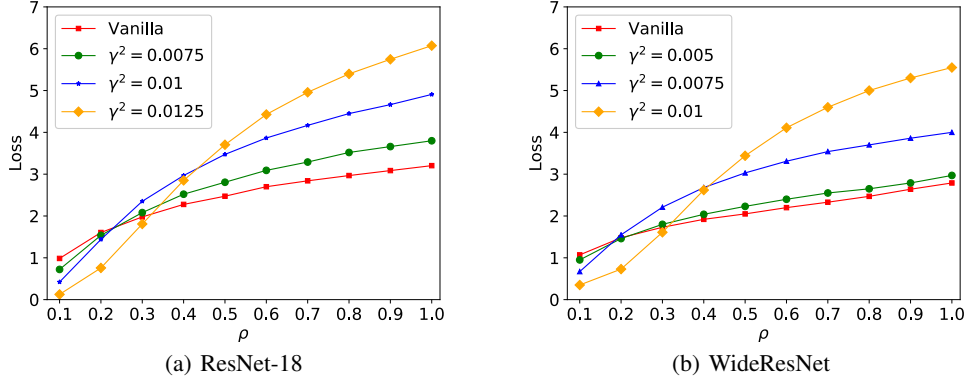
Figure 2: The effect of Gaussian noise for loss value. The red line (vanilla) represents the loss function L(w + \rho \frac{g(w)}{\|g(w)\|}) with \rho value increasing. The other three lines show the change of loss function with random initialization L(\hat{w} + \rho \frac{g(\hat{w})}{\|g(\hat{w})\|}) when increasing \rho value, where \hat{w} = w + \delta_0 . Noted that \delta_0 is from the Gaussian distribution with three different standard deviation ( \gamma^2 = 0.0075, 0.01, 0.0125 ). We select the checkpoint of 200-th epoch on CIFAR-100 as the weight w to plot the figure.
