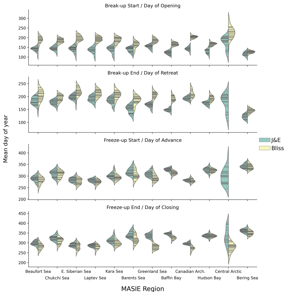
Figure 5. “Violin” plots of the Julian dates of the breakup and freeze-up metrics used in this study based on Johnson and Eicken (2016) (green shading) and the corresponding dates of ice opening, retreat, advance, and closing as defined by Bliss et al. (2019) (yellow shading). A violin plot shows a distribution by widening the horizontal lines in the ranges (of day of the year, in this case) having the highest concentration of values. The thin black lines represent the observations themselves; the black strips are clusters of lines representing groups of similar values in the distribution. The violin plots provide no information about the temporal sequence of the values.
