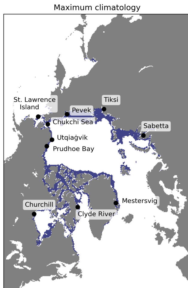
Figure 1. Landfast ice distribution shown as the maximum extent of landfast ice over the 1972–2007 period. Data source: National Ice Center via National Snow and Ice Data Center, NSIDC dataset G02172 – https://nsidc.org/data/G02172 (last access: 4 September 2022).
