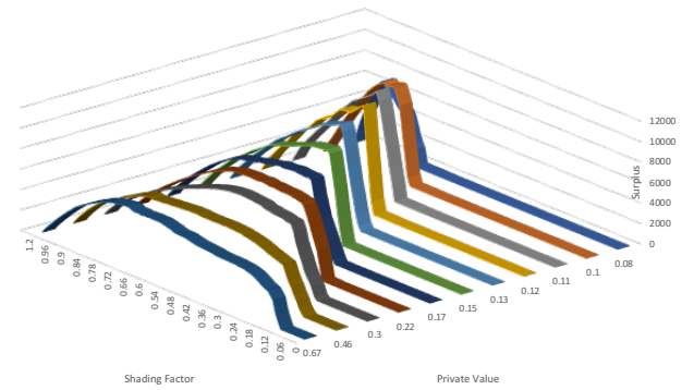
Figure 6: Predicted Surplus given Private Value and Shading Factor for one domain.
