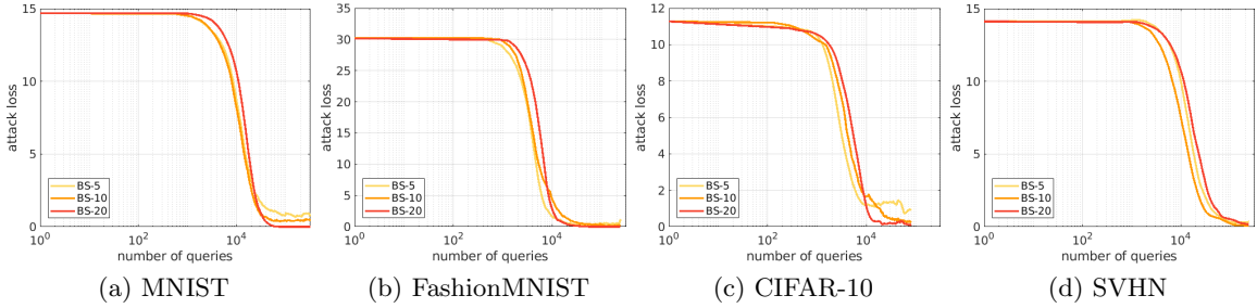
Figure 2: Impact of batch-size on our Acc-ZOM algorithm.
