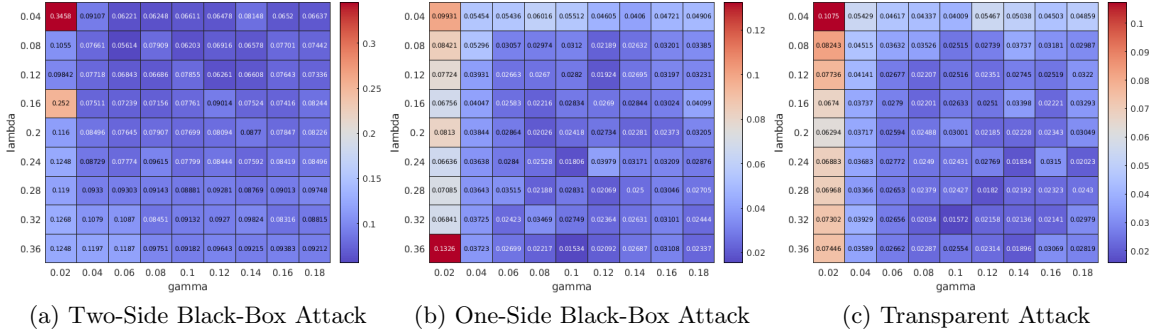
Figure 4: Stationary gap given different combinations of tuning parameters (\gamma, \lambda) .
