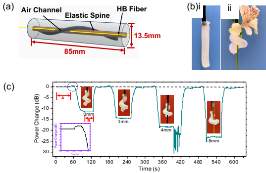
Fig. 3: (a) Detail design of the twining plant inspired soft robotic spiral gripper; (b)i. Soft spiral gripper before actuation; ii. Spiral gripper after actuation; (c) Real-time monitoring of the twining plant inspired spiral gripper using optical power measurement.
