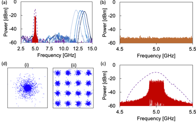
Fig. 1: (a) Transmittance of the channel as seen by the attacker (blue) and legitimate receiver (purple); (b) Sensitive signal is destructively interfered at the attacker's hand; (c) Sensitive signal is received successfully at the designated receiver; (d) Constellation diagrams seen by (i) the attacker (ii) legitimate receiver.
