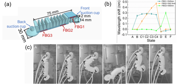
Fig. 4: (a) Inchworm-inspired soft robotic climber design; (b) Measured wavelength shift of the three FBGs at different states with respect to state A; (c) Step by step motion of the robot climbing up a 90° vertical glass wall.
