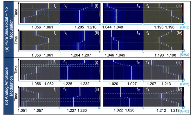
Fig. 2: Spectral waterfall of the Eigenmannia inspired photonic based jamming avoidance response. Yellow shade: jammer moving in different spectral direction. (a) single tone jamming and reference signals; (b) analog modulation for both jamming and reference signals.
